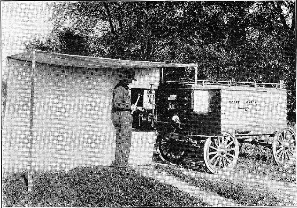
FIG. 32.—Spare parts trailer, road side set up
