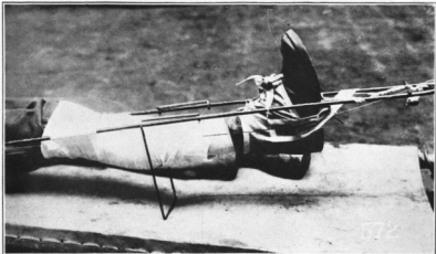
FIG. 69.—Cloth gaiter, applied over shoe for extension.
