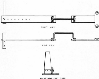
FIG. 20.—Mechanical drawing of long Lister splint with interrupting bridge of iron wire
