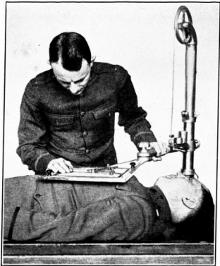
FIG. 137.—Method of showing fluoroscopic adapter with Hirtz compass
