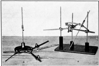
FIG. 136.—Accessory apparatus for fluoroscopic work with Hirtz compass. A, Auxiliary compass, pedestal support, and three markers with friction clips; B, Hirtz compass mounted with the three legs at different levels, so that a pointer reaches white spot on the base plane at the center of the sphere of which the curved arc is a part
