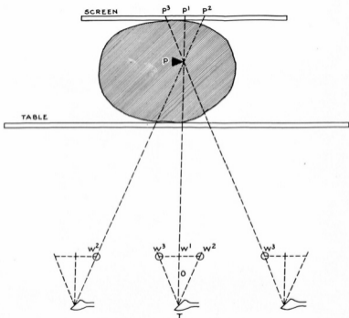
FIG. 127.—Method of similar triangles (double-shift, fixed-angle method)
