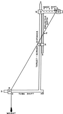
FIG. 125.—Wall meter, or indicator, for tube shift method, also showing method of using adjustable double-slider caliper
