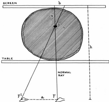
FIG. 124.—Classical single-shift triangulation method
