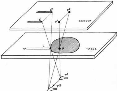
FIG. 106—Diagrammatic representation of the parallax method
