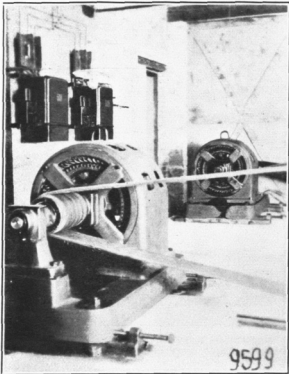
FIG. 100.—Motors of 25 horsepower, used to drive compressors
