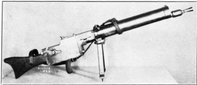
FIG. 64.—German 08/15 (Spandau) machine gun
