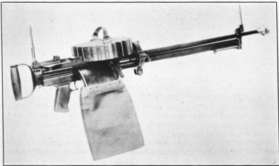
FIG. 61.—Lewis aircraft machine gun, model 1917, caliber .30
