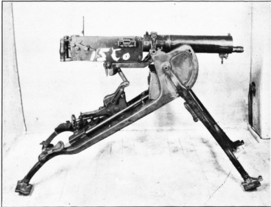
FIG. 54.—German Maxim machine gun on mount
