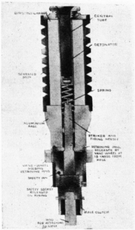
FIG. 32.—Longitudinal section of an English grenade
