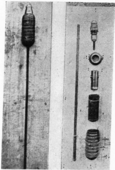
FIG. 29.—German combination grenade for hand or rifle use
