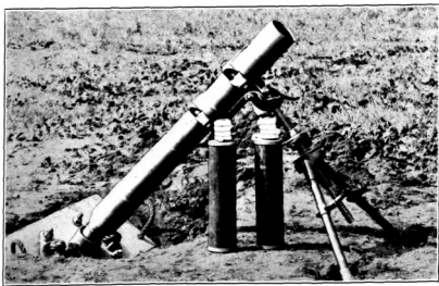
FIG. 26.—Stokes 4-inch trench mortar and ammunition
