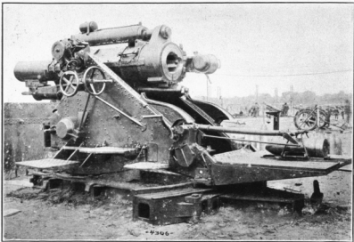
FIG. 8.—British 9.2-inch howitzer, model 1917. This gun shoots a shell weighing 290 pounds 8,690 meters
