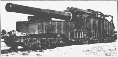
FIG. 6.—United States 14-inch railway artillery. This type was evolved entirely by the United States Ordnance Department. It is an excellent weapon for coast defense and hurls a 1,200-pound projectile more than 18 miles.
