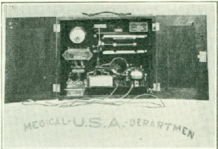
FIG. 77.—Galvanic and slow sinusoidal apparatus, with meter and rheostat (Wappler)
