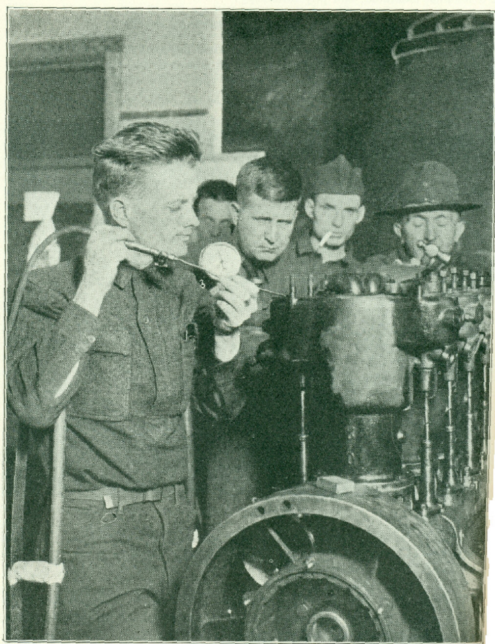
FIG. 19.—An invalid instructor in oxyacetylene welding
